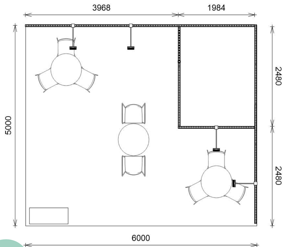
TOP VIEW
